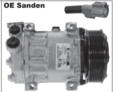
OE Sanden 300-4248 Aftmkt 300-4255 OE# SKI4417, SKI4818
